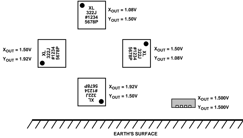
Figure 22. Output Response vs. Orientation
